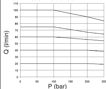
BACK PRESSURE ON SECONDARY LINE
