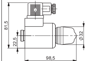
EMERGENCY (COILS WITH HIRSCHMANN CONNECTION)
