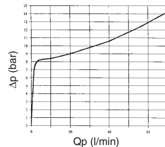
AM.5.H.3V.P1... \Delta P - PUMP FLOW CURVE
