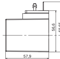
EMERGENCY (COILS WITH HIRSCHMANN CONNECTION)
