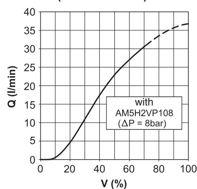
(36 l/min P \rightarrow A/B)
