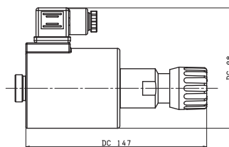
ROTARY WITHOUT CONNECTOR (P2) ROTAN ROTARY WITH CONNETOR (P1)
