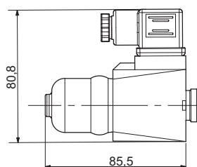
MANUAL WITHOUT CONNECTOR (ES) MANUAL WITH CONNECTOR (E1)
