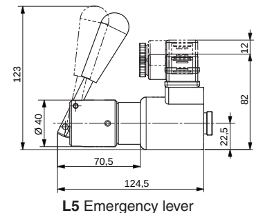
L5 Emergency lever
