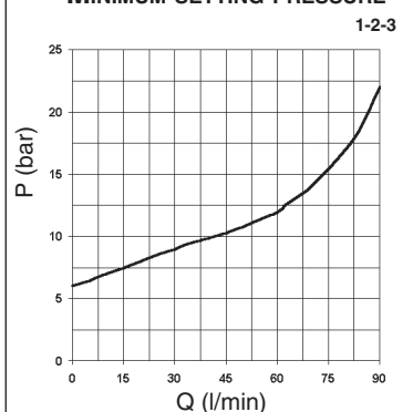
PVS.5... / PVS.U.5... MINIMUM SETTING PRESSURE 1-2-3
