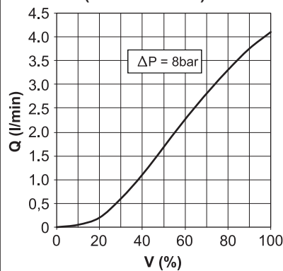
(15 l/min P \rightarrow A/B)
